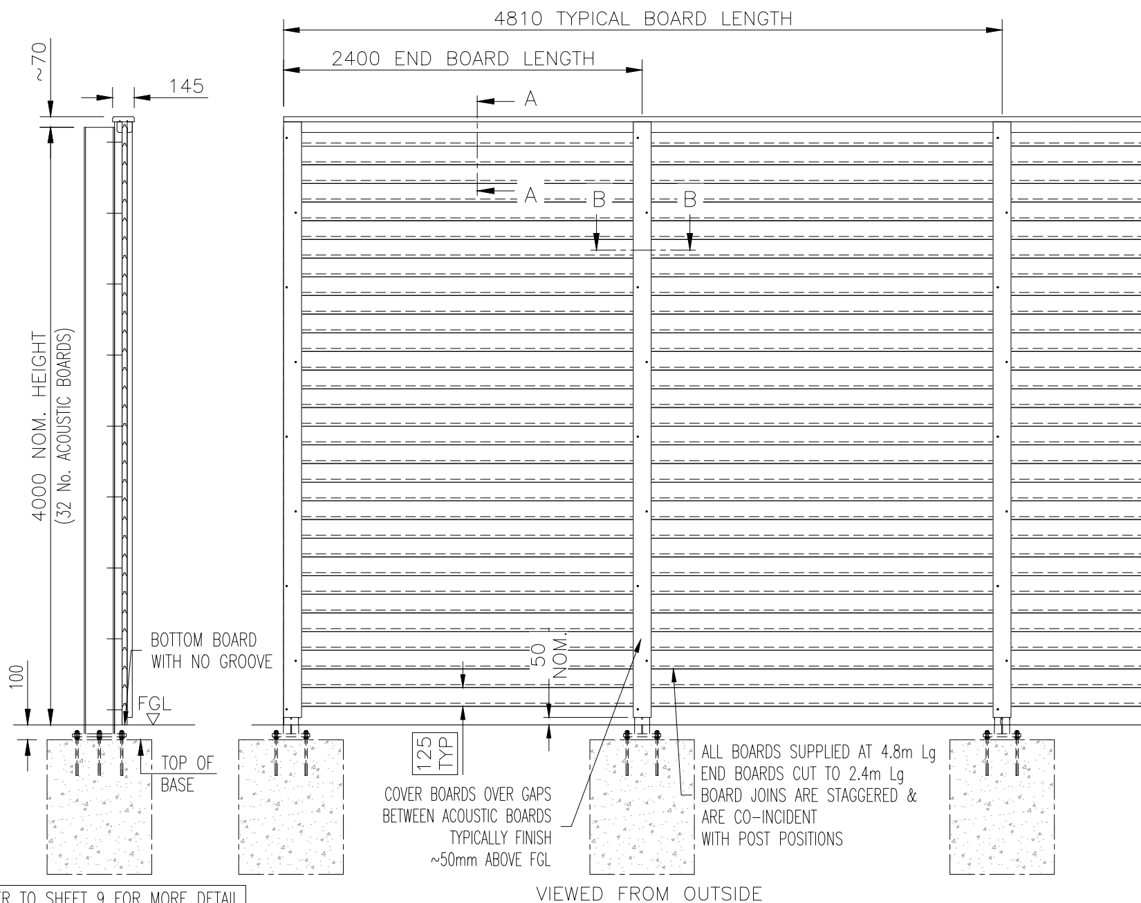
JAKOUSTIC HIGHWAY FENCE – BASEPLATED (WITH CAPPING) – 4m HIGH
