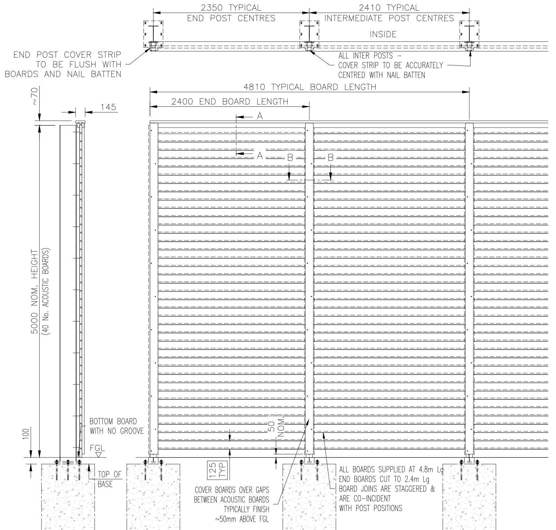
JAKOUSTIC HIGHWAY FENCE – BASEPLATED (WITH CAPPING) – 5m HIGH
