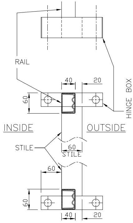
VIEW ON C-C HINGE BOX DETAIL (HANDED FOR OPPOSITE LEAF)
