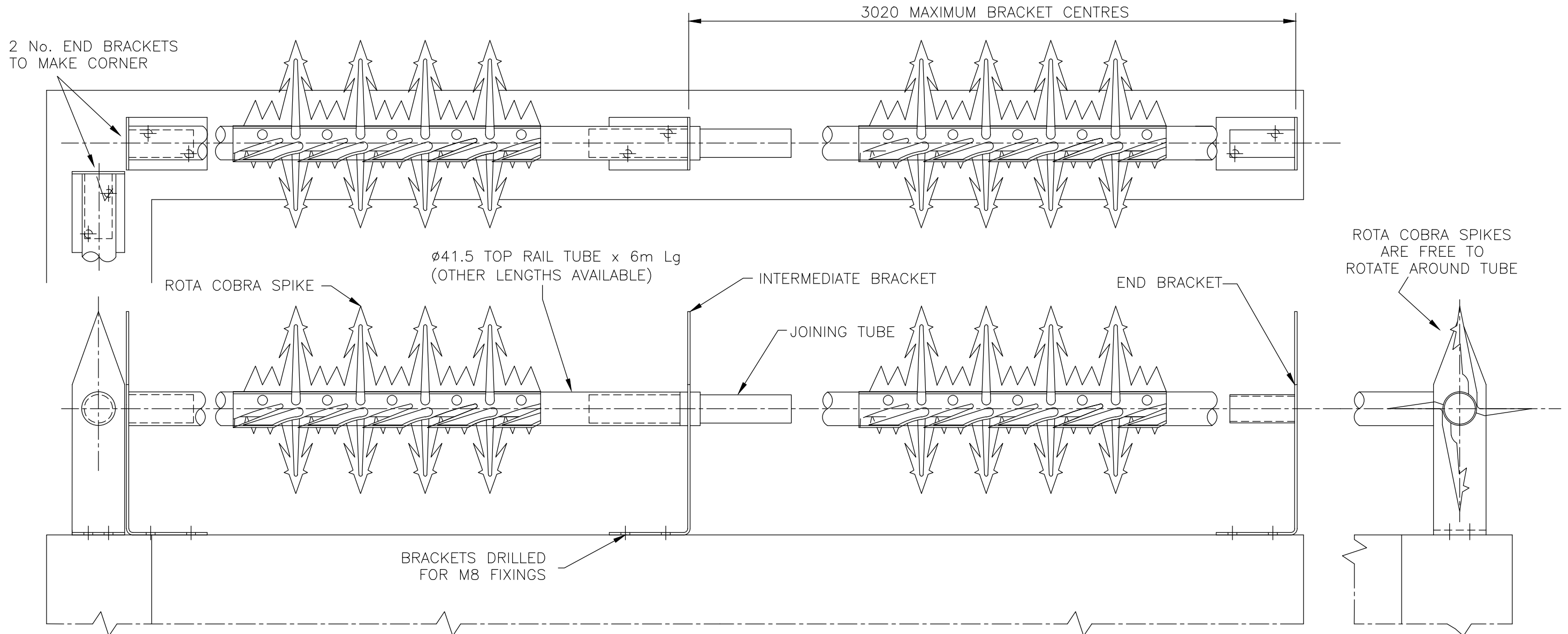
ROTARY COBRA SPIKE – MOUNTED TO WALL TOP
