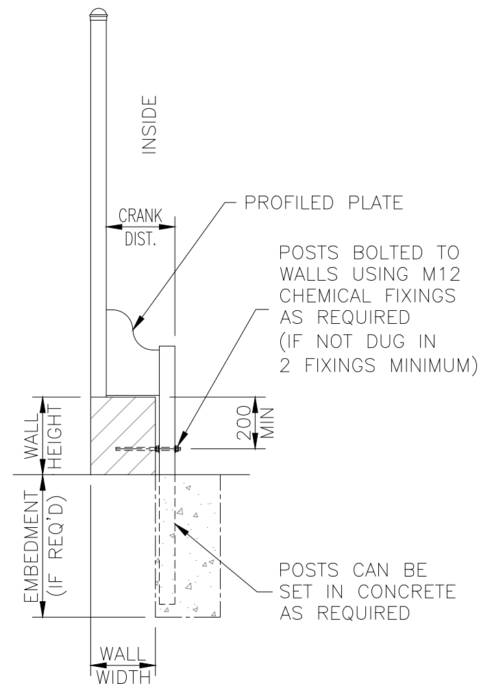
OPTION 'A' ROUND POSTS
