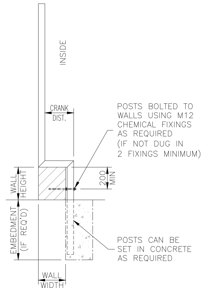
OPTION 'B' SQUARE POSTS
