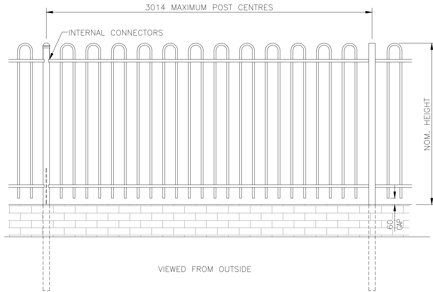
OPTION 'A' ROUND POST
