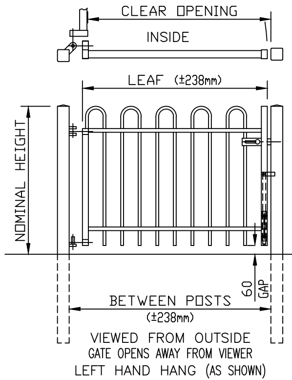
BOWTOP PEDESTRIAN SINGLE GATE
