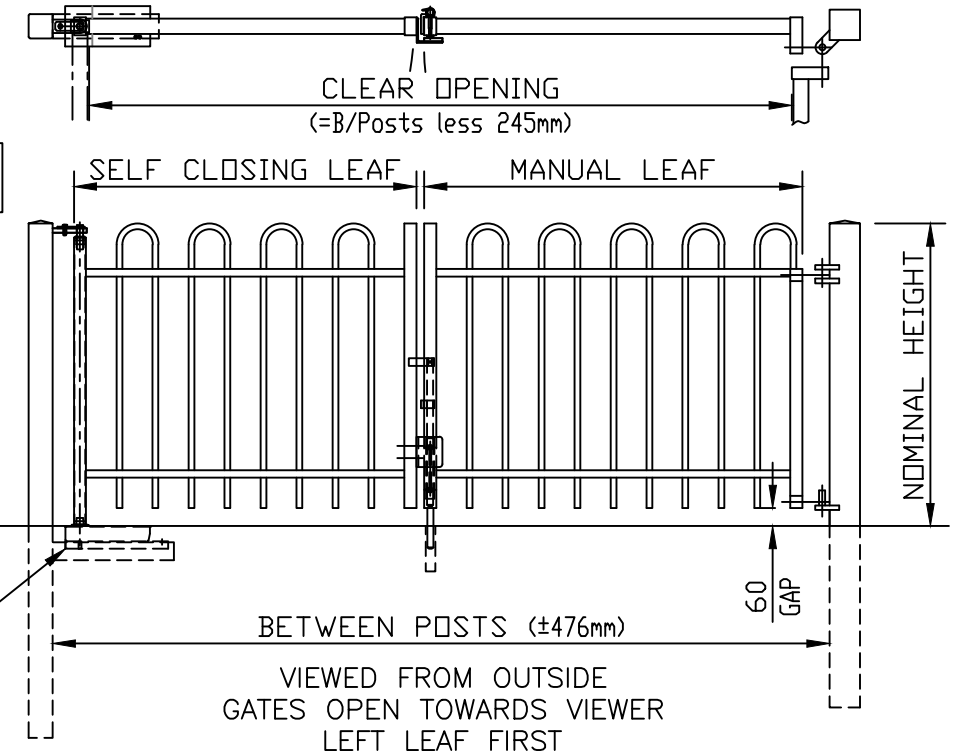
BOWTOP COMBINATION DOUBLE GATE – SELF CLOSER + MANUAL
