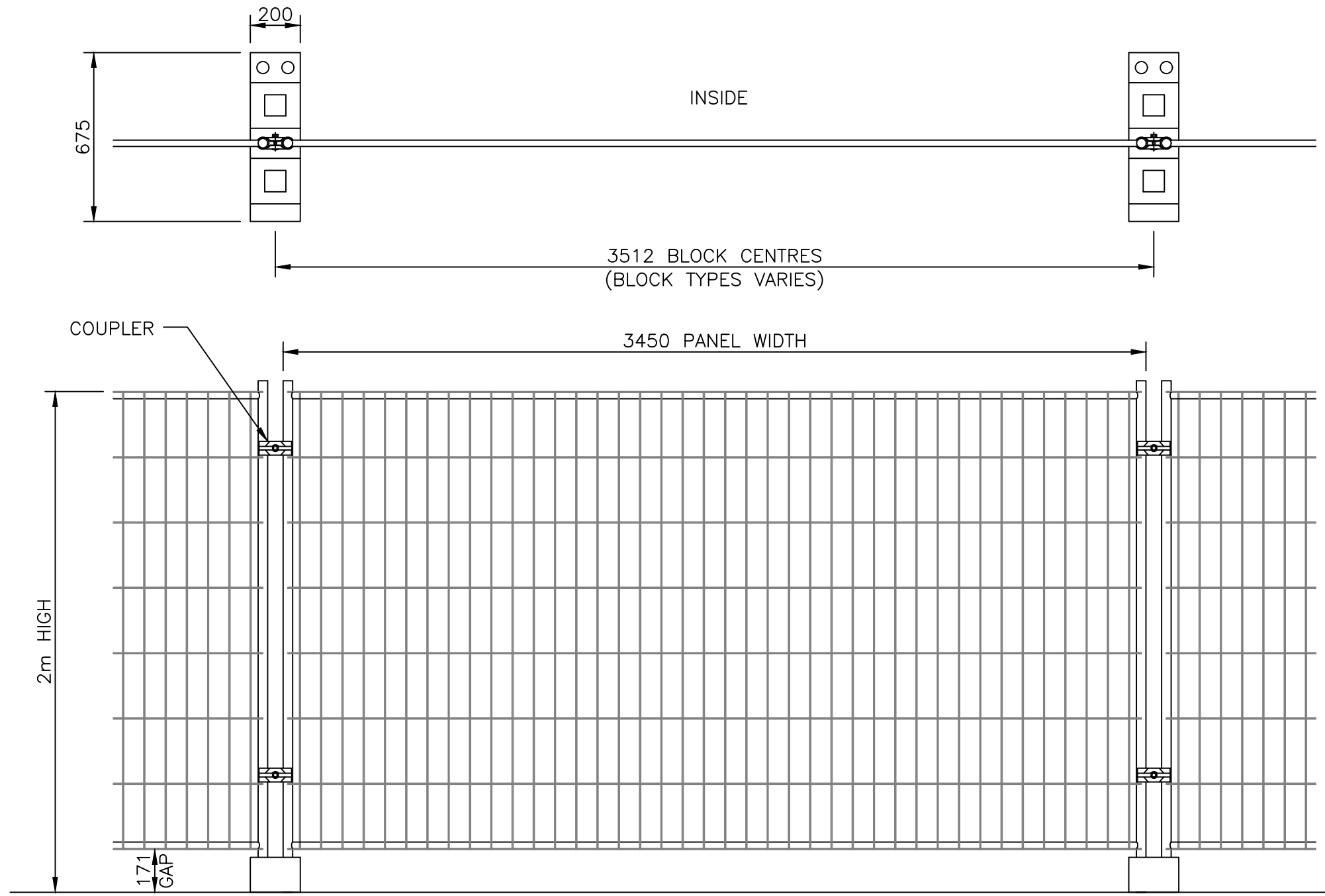
VIEWED FROM OUTSIDE EXPRESS TEMPORARY FENCE
