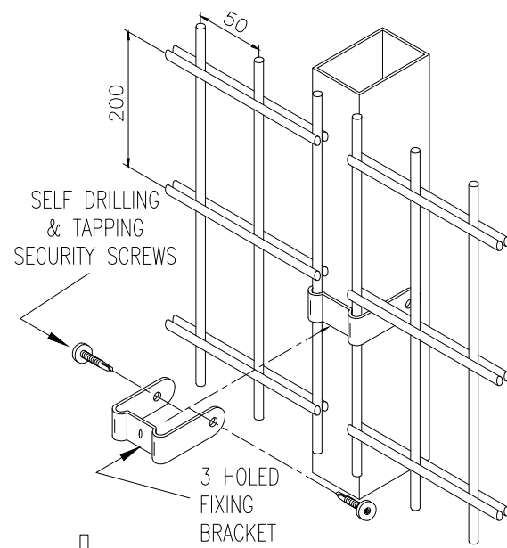
FIXING DETAILS
