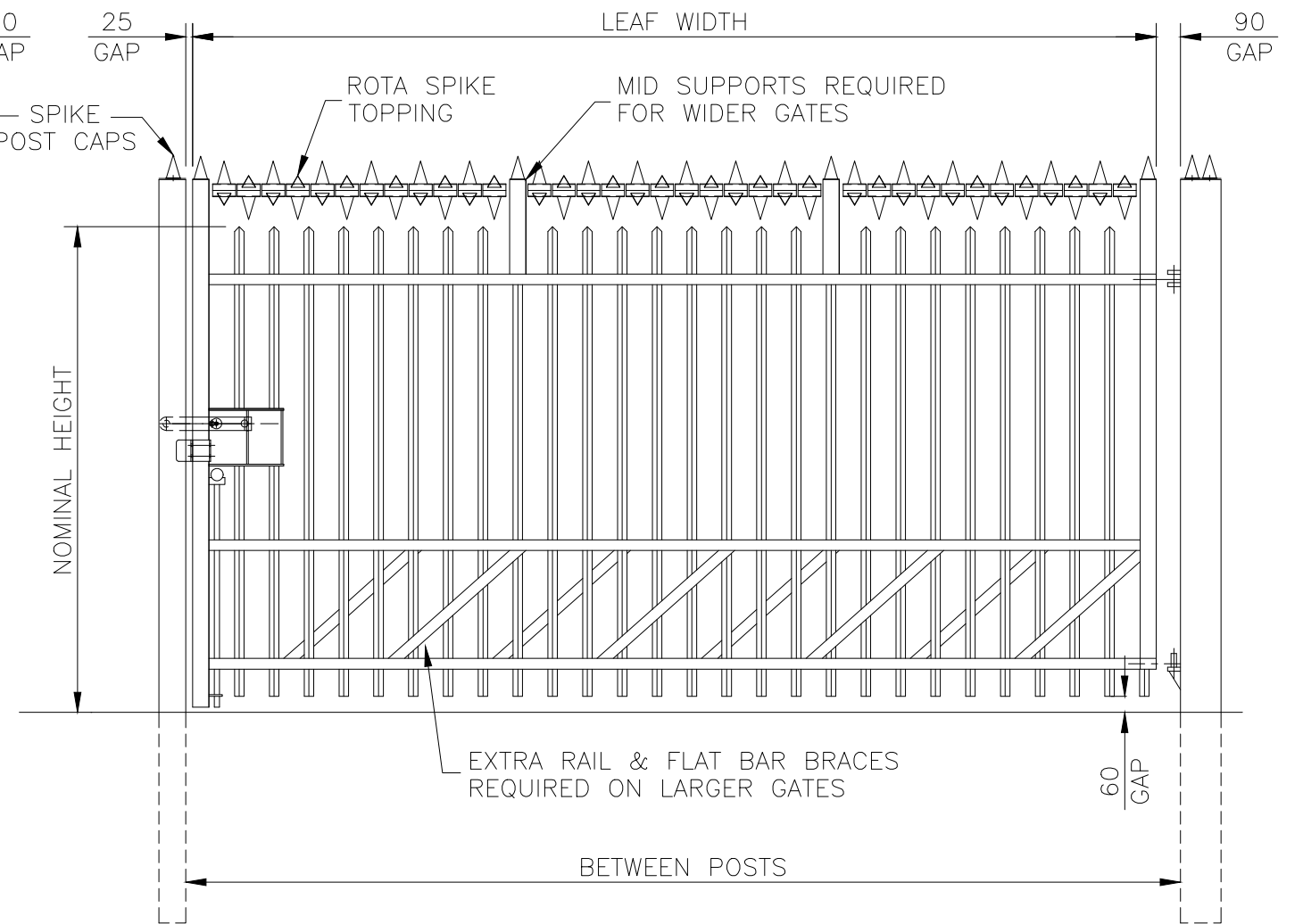
VIEWED FROM OUTSIDE GATE OPENS AWAY FROM VIEWER RIGHT HAND HANG AS SHOWN
