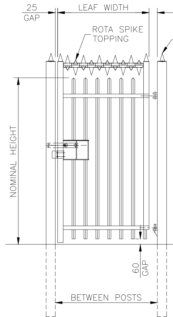
VIEWED FROM OUTSIDE GATE OPENS AWAY FROM VIEWER RIGHT HAND HANG AS SHOWN
