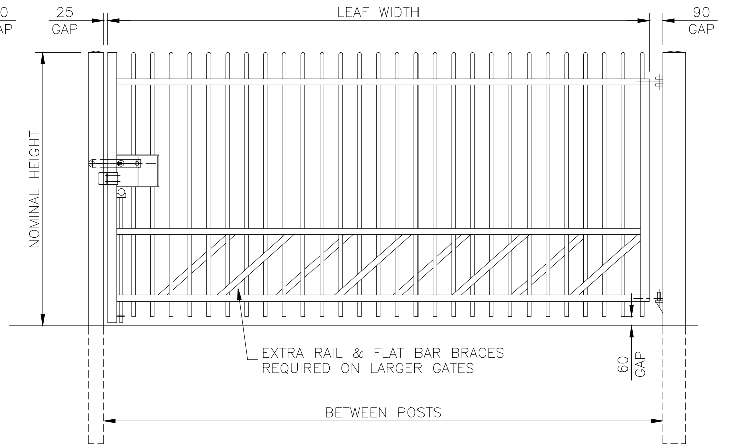
VIEWED FROM OUTSIDE GATE OPENS AWAY FROM VIEWER RIGHT HAND HANG AS SHOWN 124 PALE PITCH (AS DRAWN)
