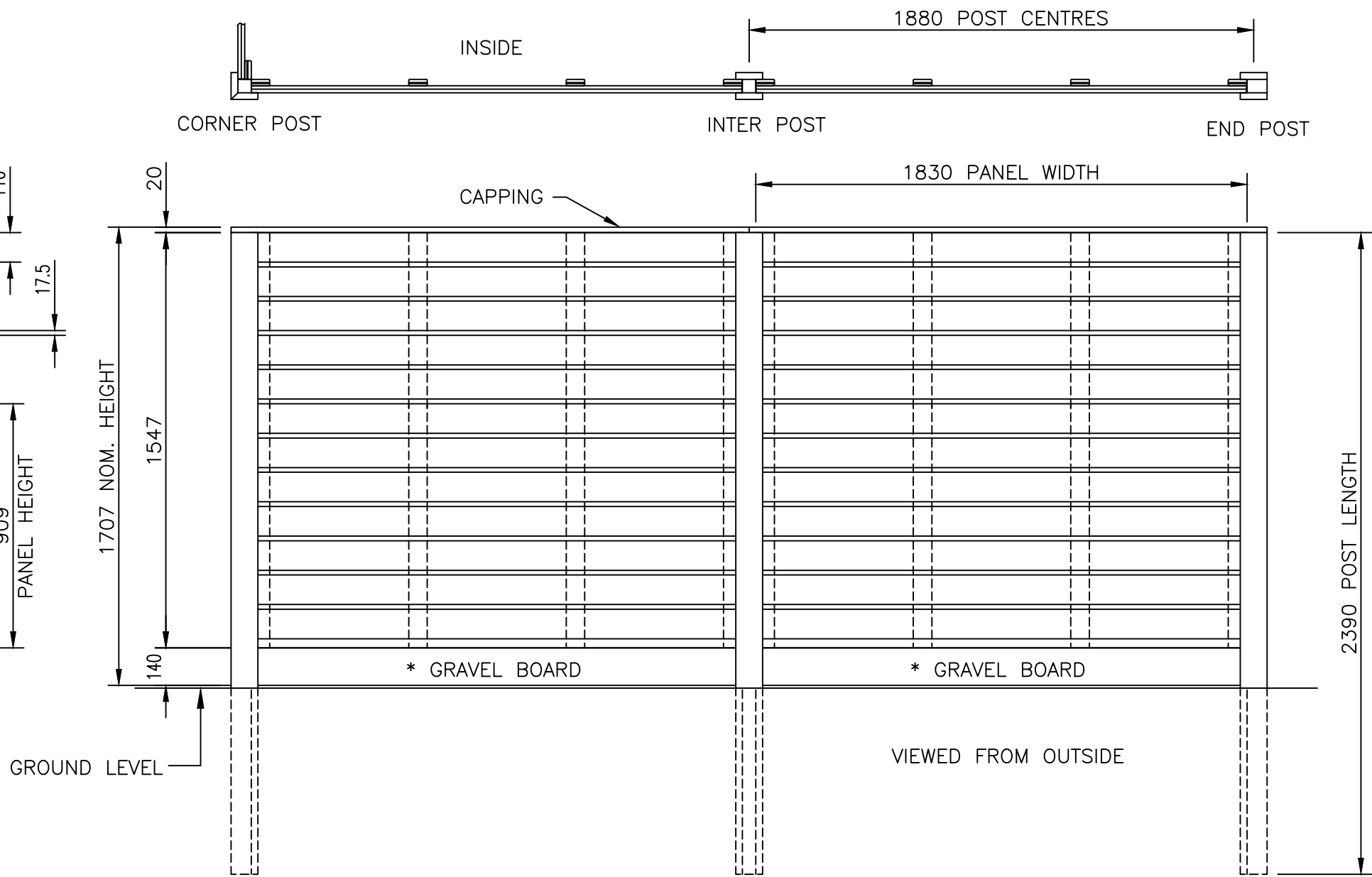
SHADOWLINE FENCE WITH SLOTTED POSTS
