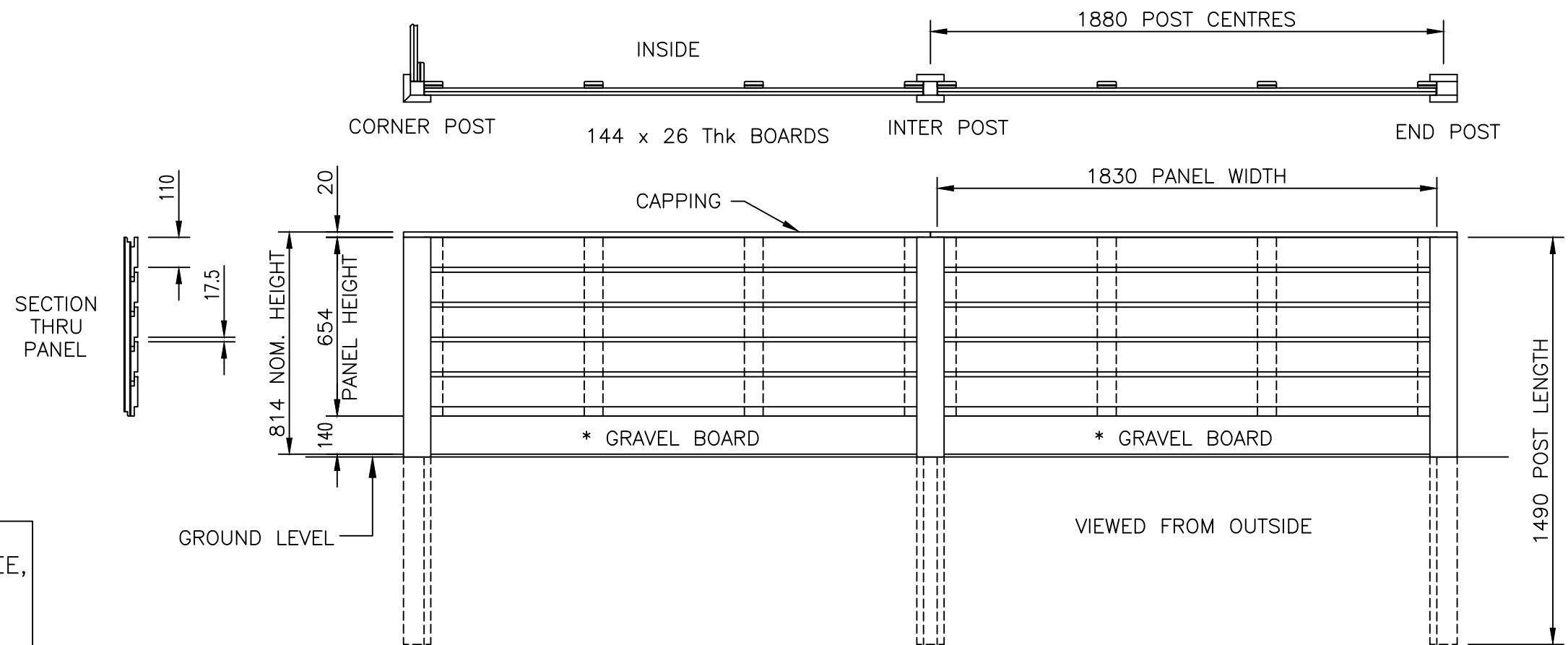
SHADOWLINE FENCE WITH SLOTTED POSTS
