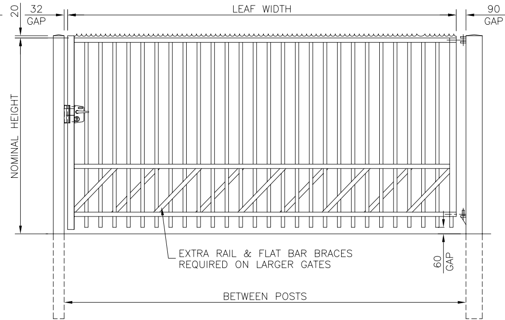
VIEWED FROM OUTSIDE GATE OPENS AWAY FROM VIEWER RIGHT HAND HANG AS SHOWN
