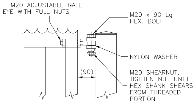
TOP HINGE DETAIL (SCALE 1:8)
