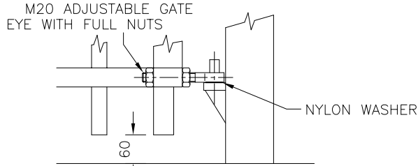
BOTTOM HINGE DETAIL (SCALE 1:8)
