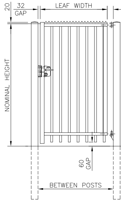
VIEWED FROM OUTSIDE GATE OPENS AWAY FROM VIEWER RIGHT HAND HANG AS SHOWN
