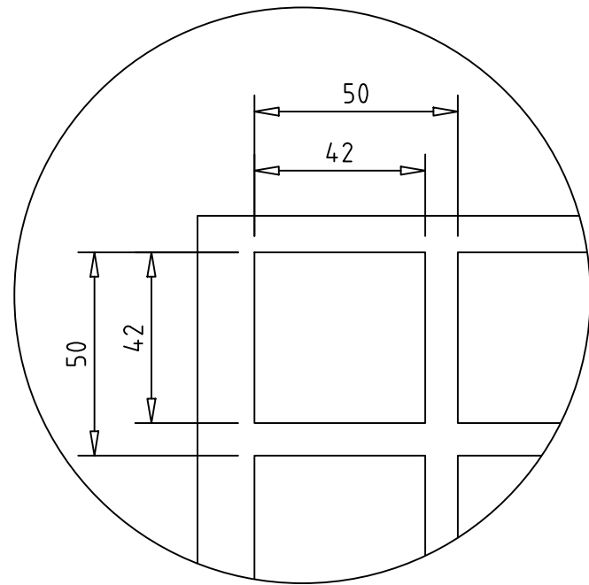
MESH DETAIL
