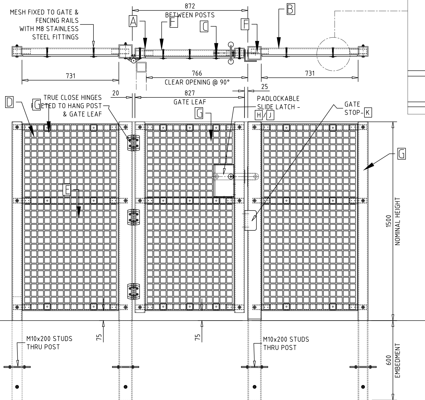
GATE & SIDE PANELS VIEWED FROM OUTSIDE GATE OPENS TOWARDS VIEWER
