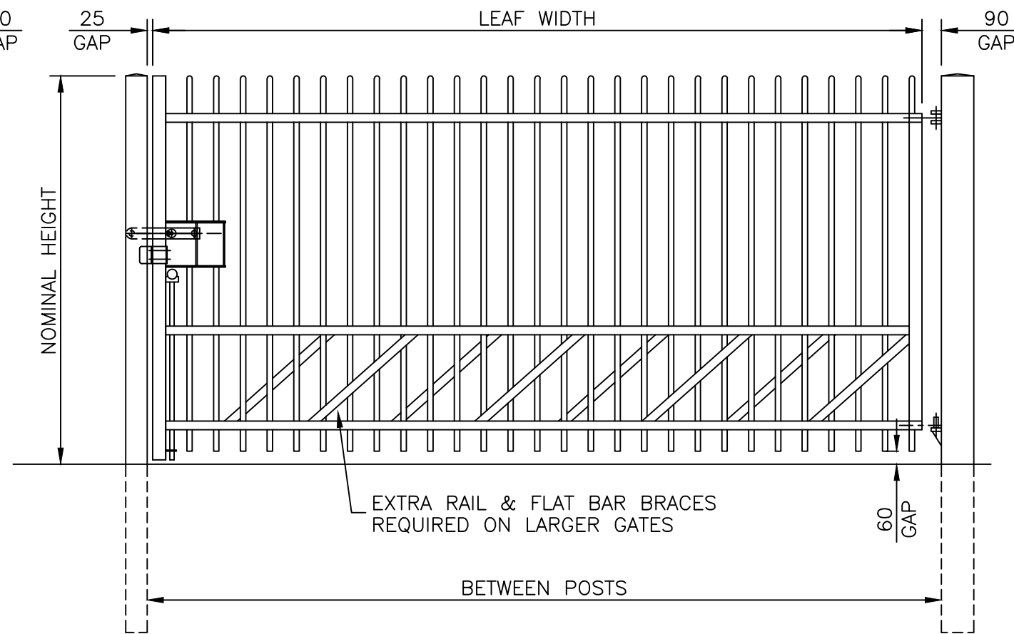
VIEWED FROM OUTSIDE GATE OPENS AWAY FROM VIEWER RIGHT HAND HANG AS SHOWN 124 PALE PITCH (AS DRAWN)
