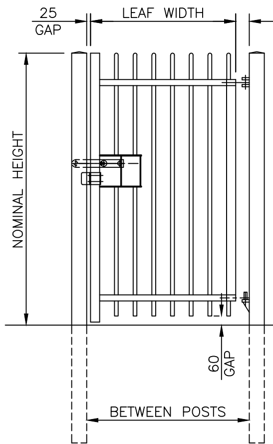
VIEWED FROM OUTSIDE GATE OPENS AWAY FROM VIEWER RIGHT HAND HANG AS SHOWN 124 PALE PITCH (AS DRAWN)
