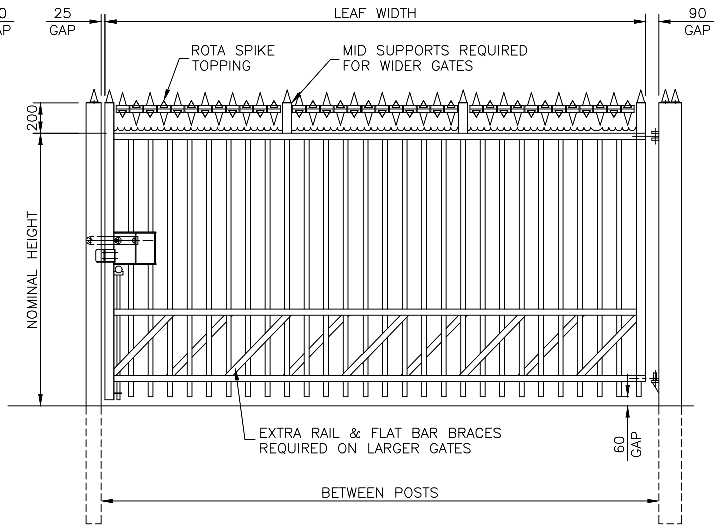
VIEWED FROM OUTSIDE GATE OPENS AWAY FROM VIEWER RIGHT HAND HANG AS SHOWN
