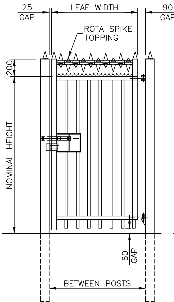
VIEWED FROM OUTSIDE GATE OPENS AWAY FROM VIEWER RIGHT HAND HANG AS SHOWN
