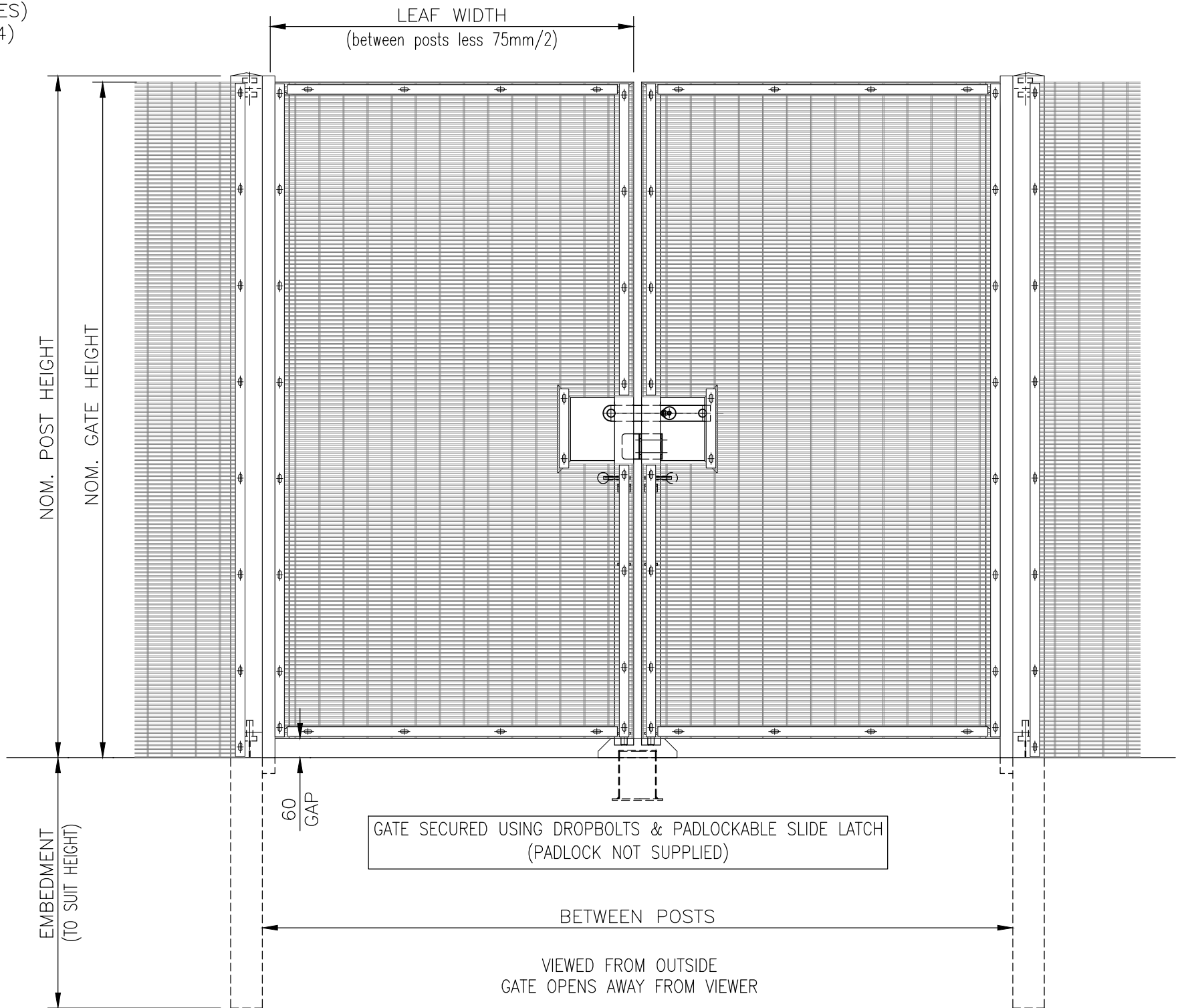
'358' SECURIMESH DETAILS
