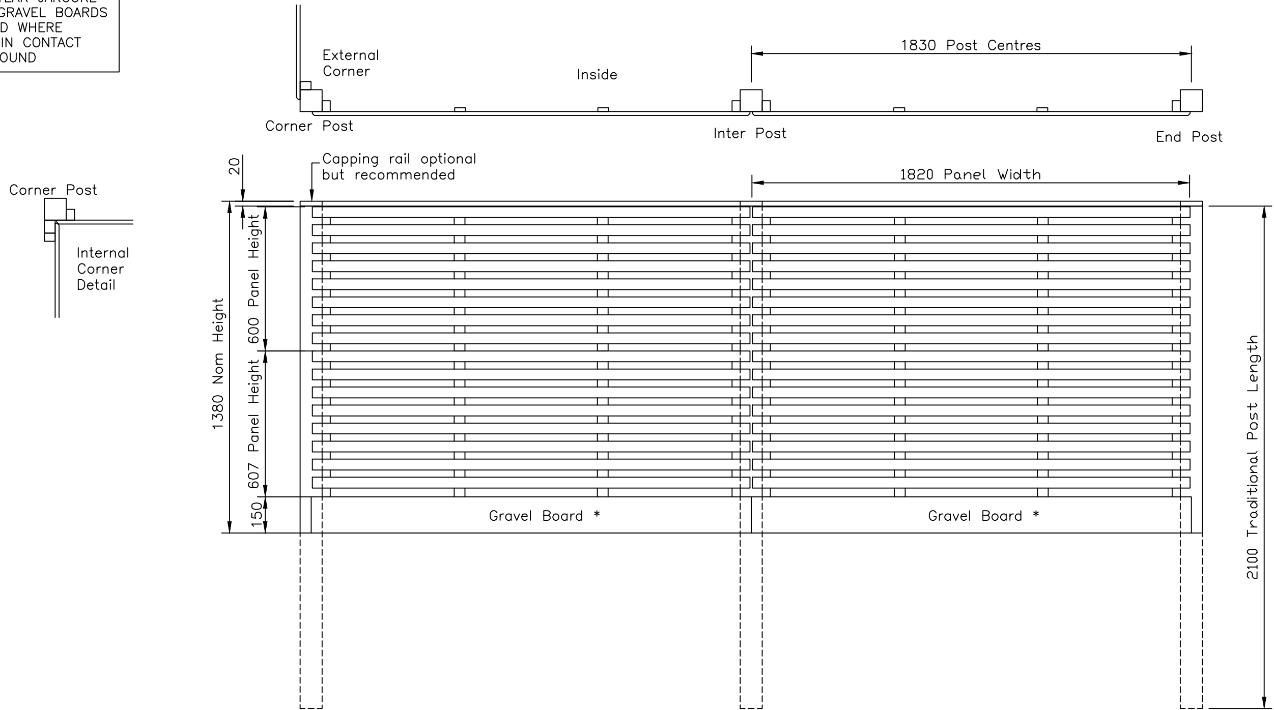
Metro Fencing with Heavy Duty Panel Posts Viewed from Outside
