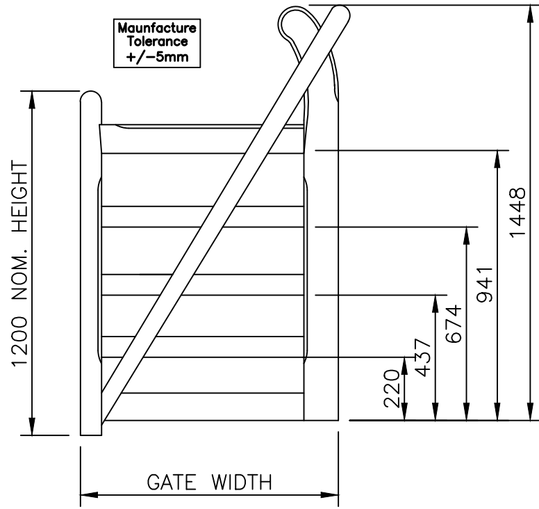
VIEWED FROM OUTSIDE GATE RIGHT HAND HANGING. PLEASE STATE HAND REQUIRED. (AUTOMATED)
