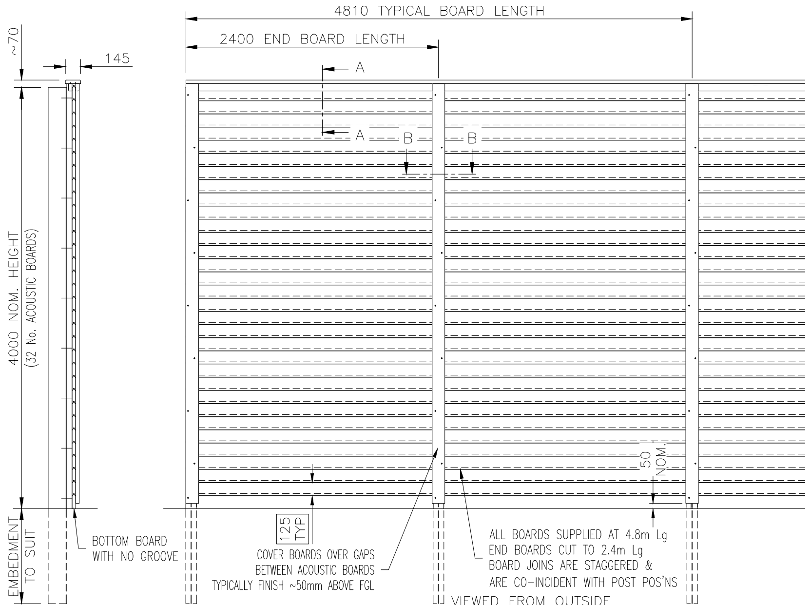
JAKOUSTIC HIGHWAY FENCE (WITH CAPPING) – 4m HIGH
