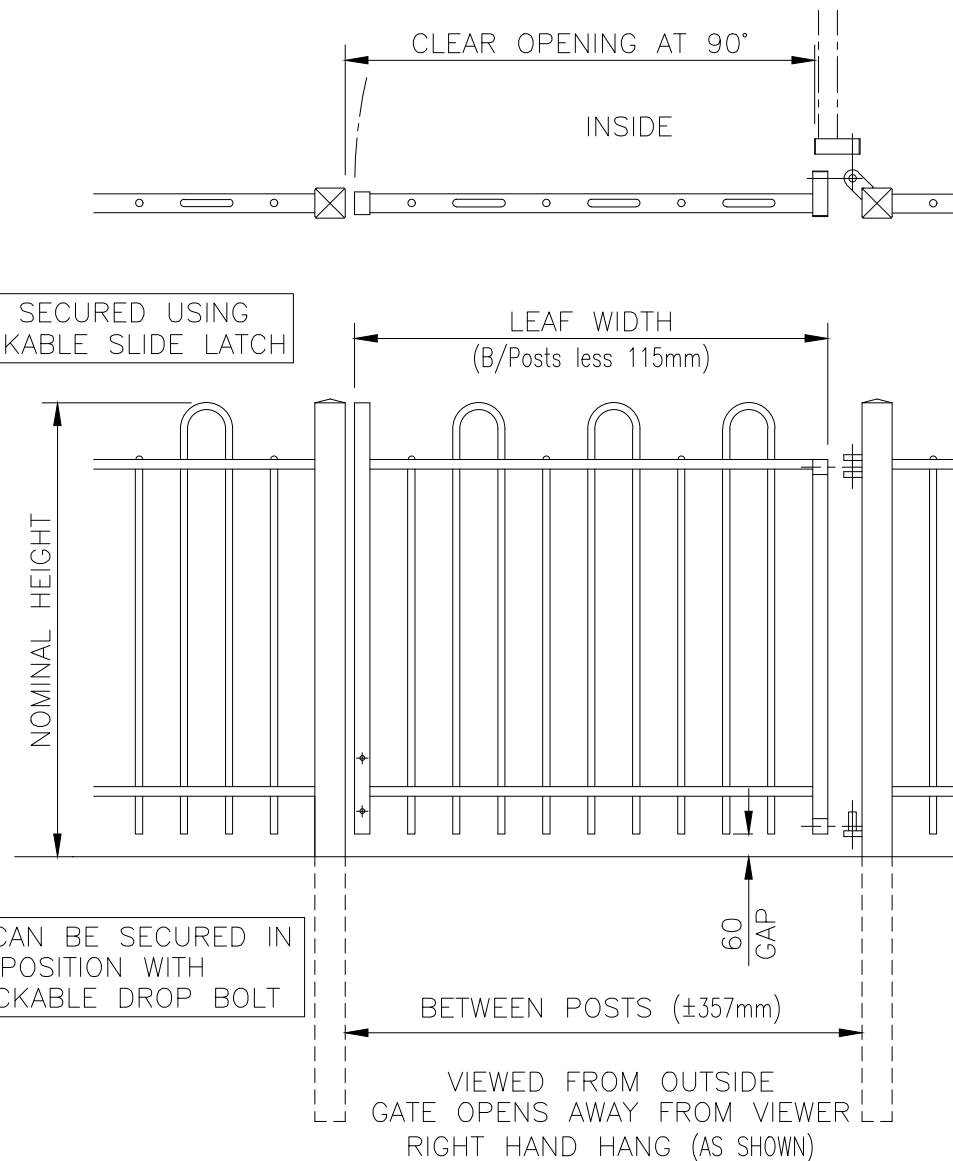
PEDESTRIAN SINGLE GATE WITH SLIDE LATCH
