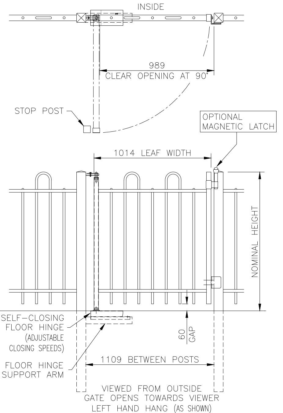
SELF CLOSING SINGLE GATE
