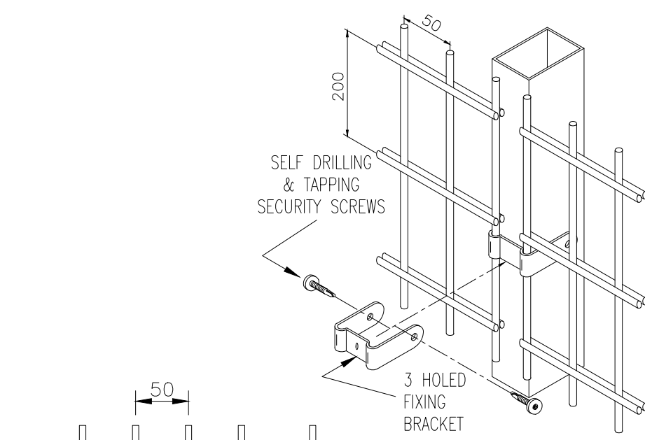
FIXING DETAILS
