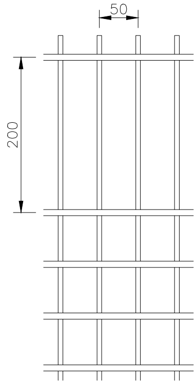
MESH DETAILS (SCALE 1:5)
