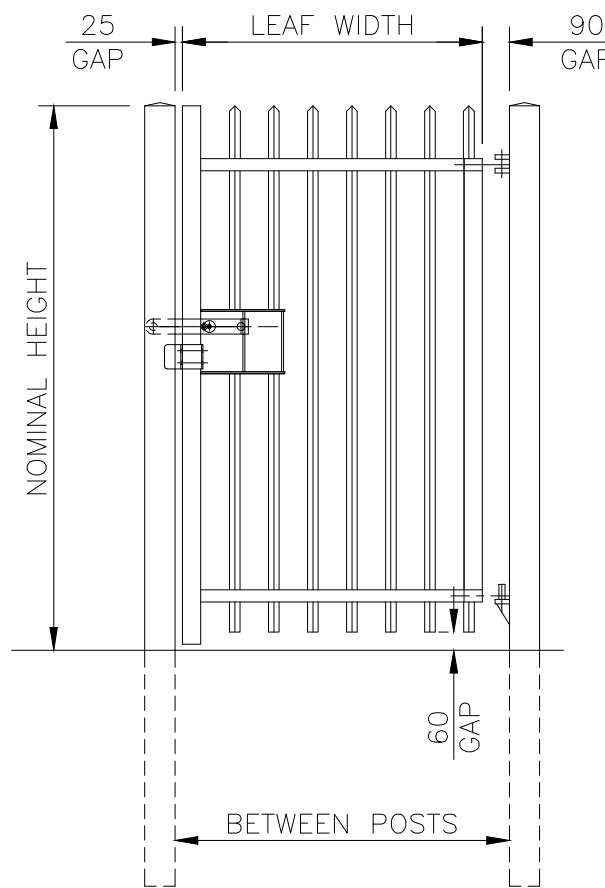
VIEWED FROM OUTSIDE GATE OPENS AWAY FROM VIEWER RIGHT HAND HANG AS SHOWN
