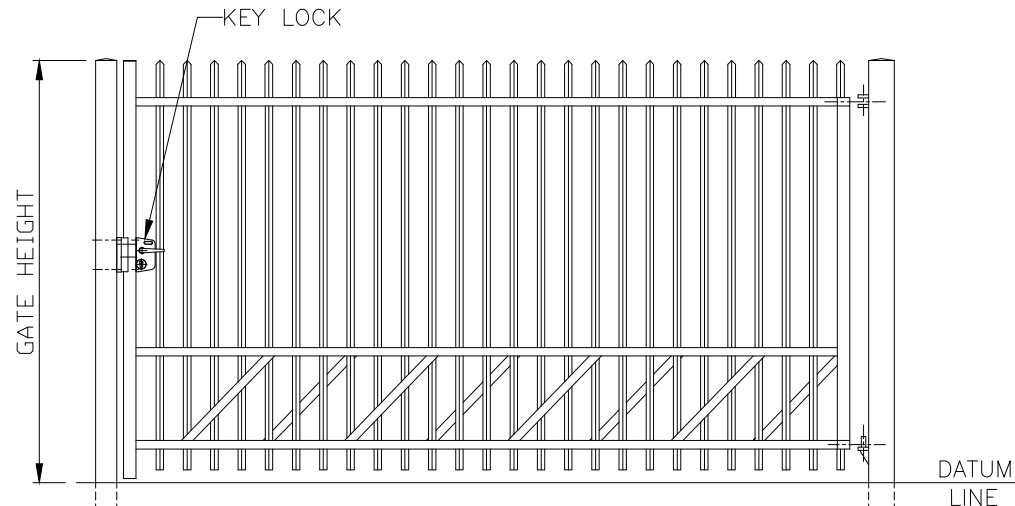
LARGE GATES i.e. 1.8M High – 2.5M High & Over 3.5M Wide
