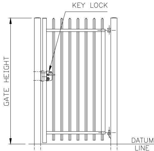
SMALL GATES i.e. Up To 2.5M High & Under 3.5M Wide
